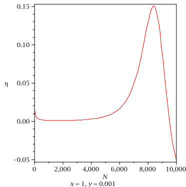
Figure: Plot of \eta against N
