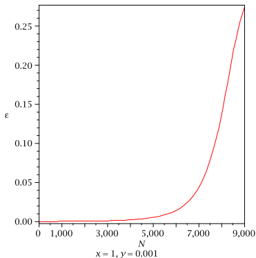
Figure: Plot of \varepsilon against N
